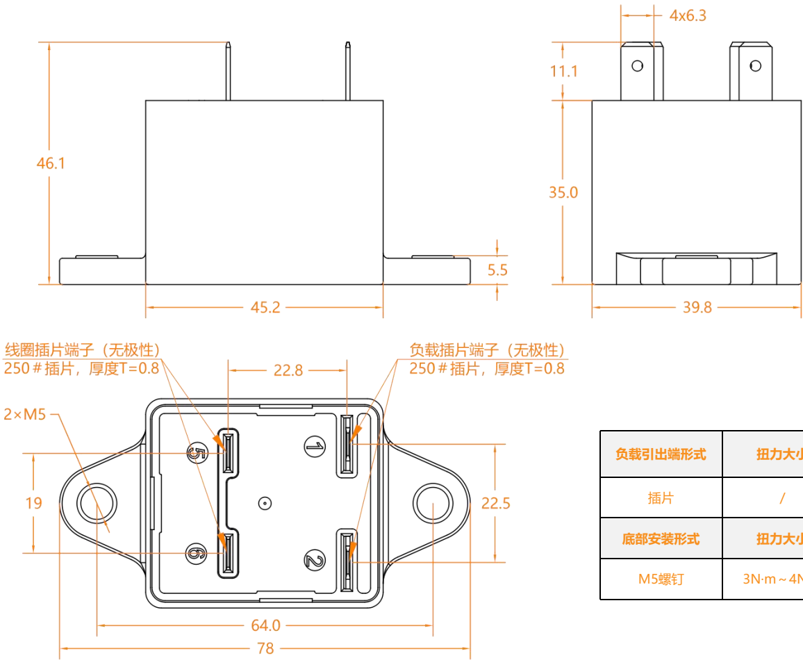
Dimensions (mm)
